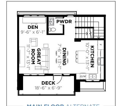
MAIN FLOOR ALTERNATE
