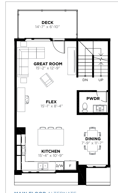
MAIN FLOOR ALTERNATE The deck door swing may vary
