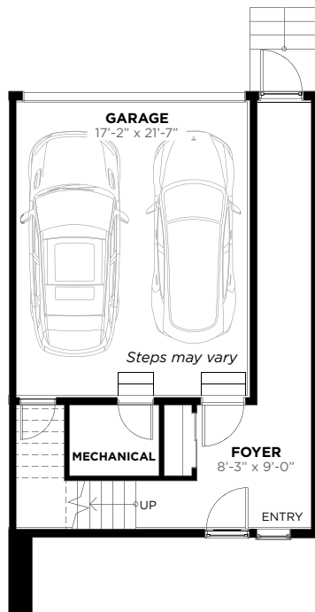
ENTRY LEVEL
