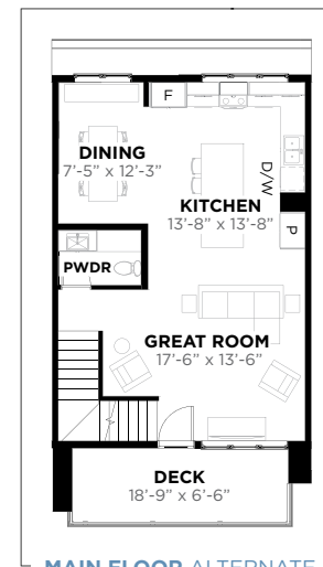
MAIN FLOOR ALTERNATE
